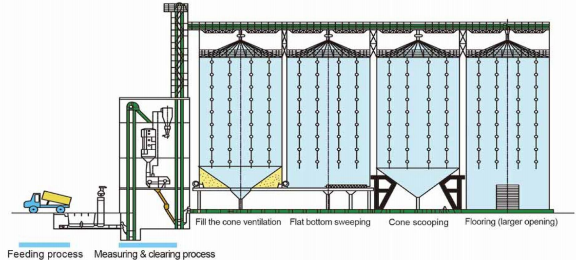
Process flow 1
