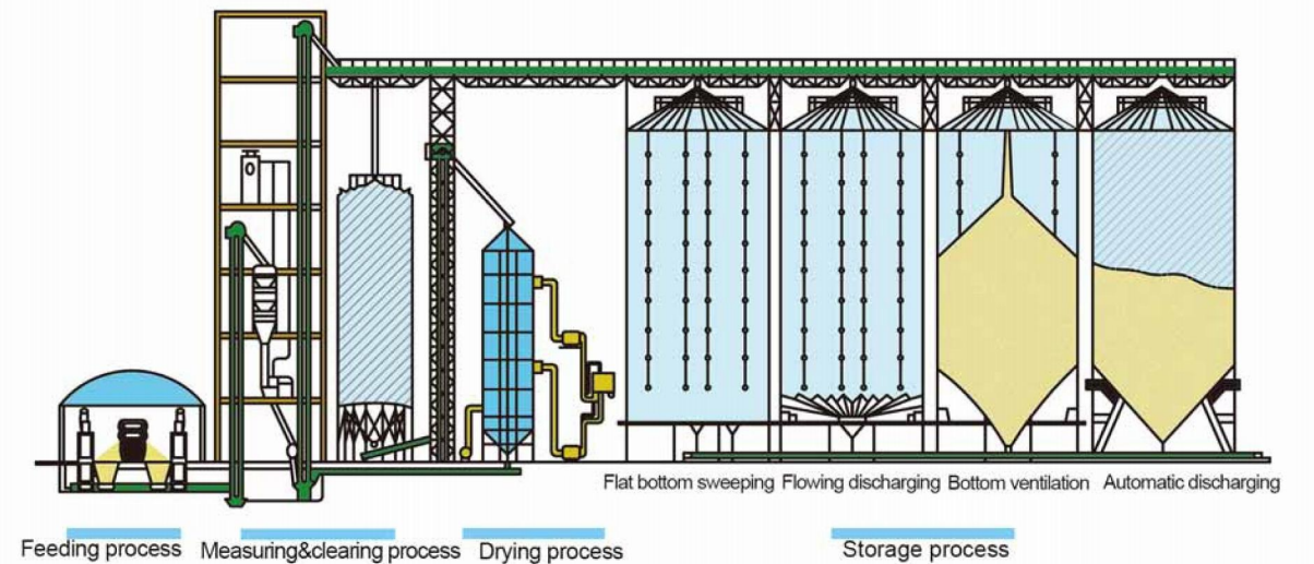
Process flow 2
