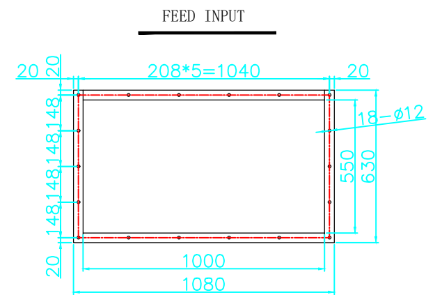
PELLET MILL YPM660
